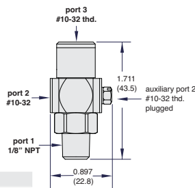
Part No. IPC-3FPN*
