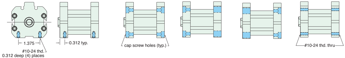
Bottom Mount AF-Bxx-24-x
