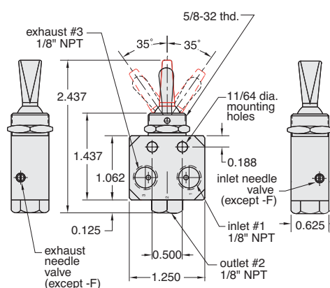
Adjustable (NP Brass Toggle shown)
