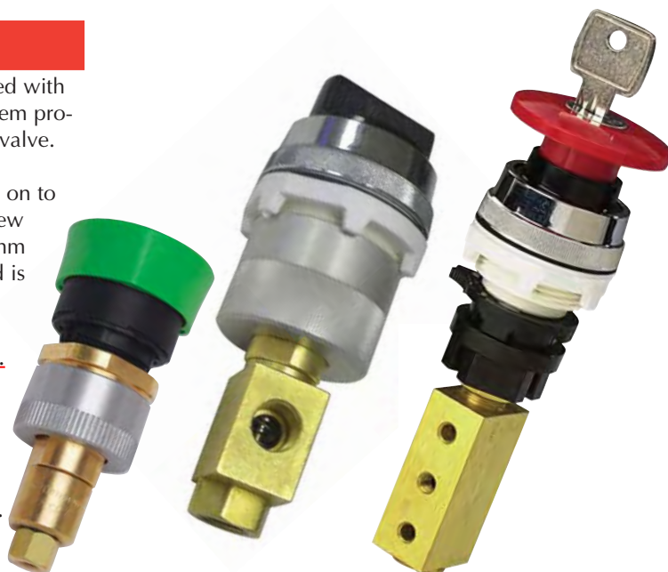
PB-22-X Adapter (22 mm) PB-30 Adapter (30 mm) PB-85 Adapter (30 mm)
