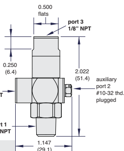
Part No. IPC-3FQF*
