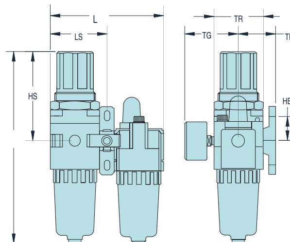
MMFRLS-3Q-D Stacking FRL with Bowl Shields and Auto Drain
