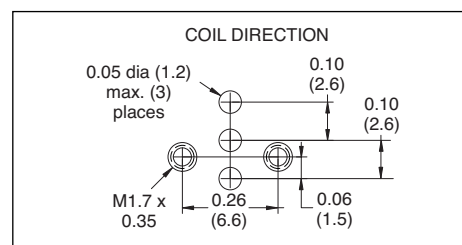
Mounting Interface
