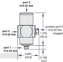
Part No. IPC-2NLN
